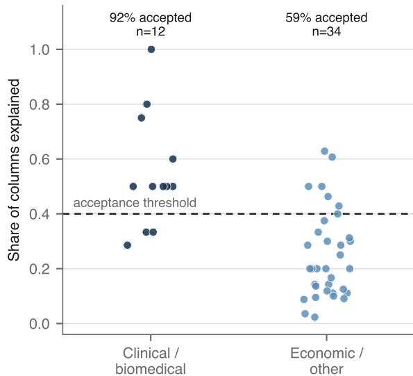
Datasets where evidence exists
