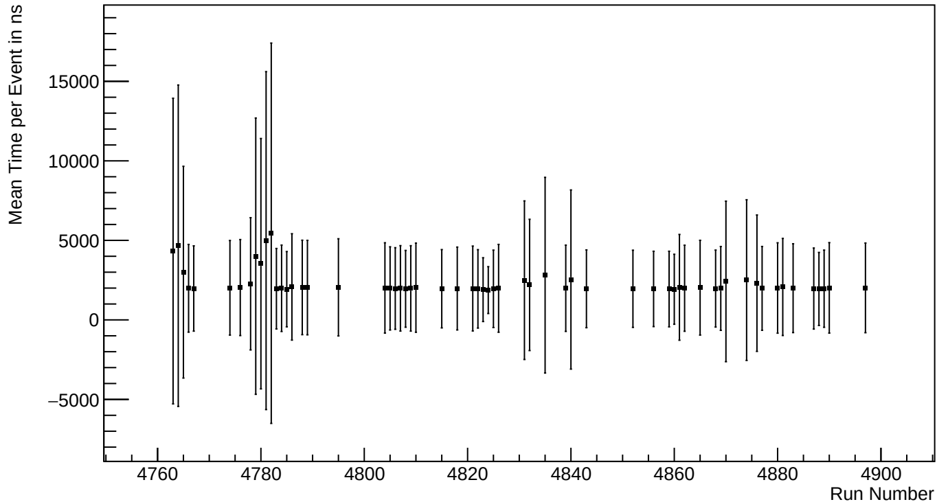
Mean Time per Event in ns In Tank
