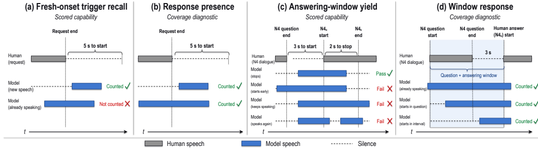
Figure 3: Schematic speech timelines for the response-timing metrics.
