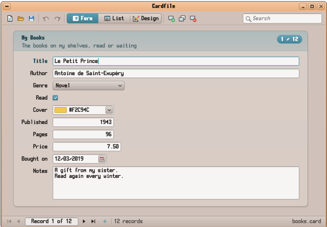
Cardfile's Form view with its sample (SD:/docs/books.card): a record on its index card.
