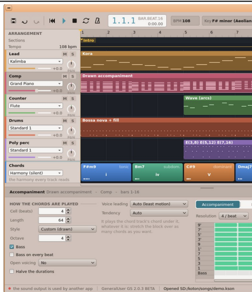
An accompaniment customised: the grid of the chord's voices.
