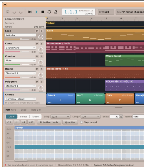
A riff over its chords: their tones shaded.
