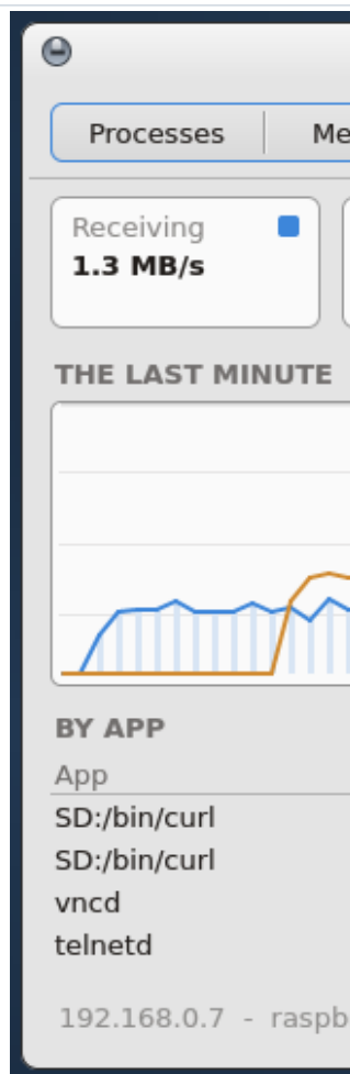
taskman — the network (on the Pi)
