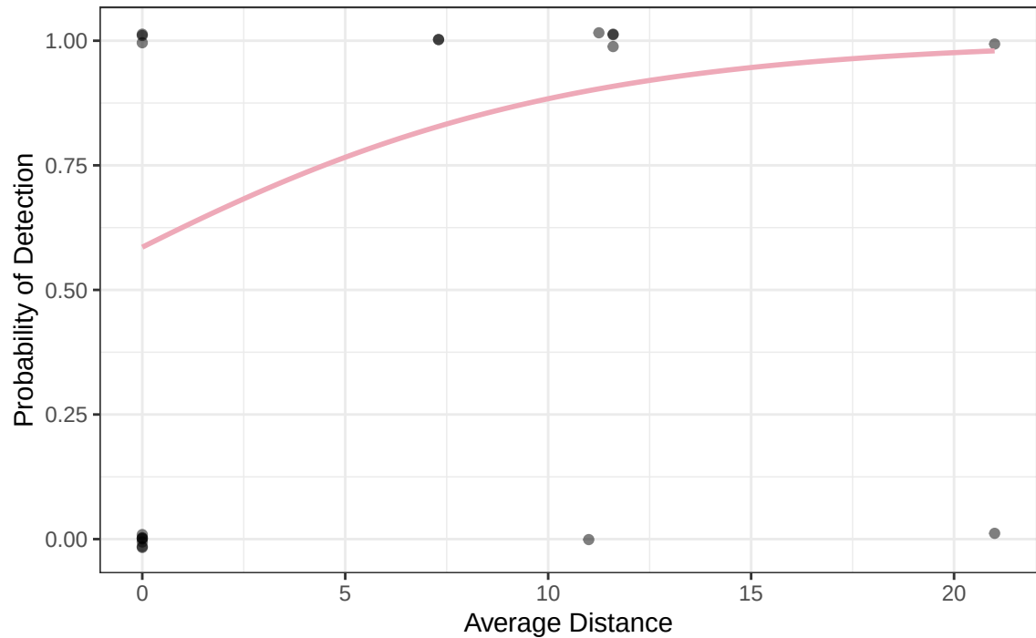
Logistic Regression Curve: Average Distance
