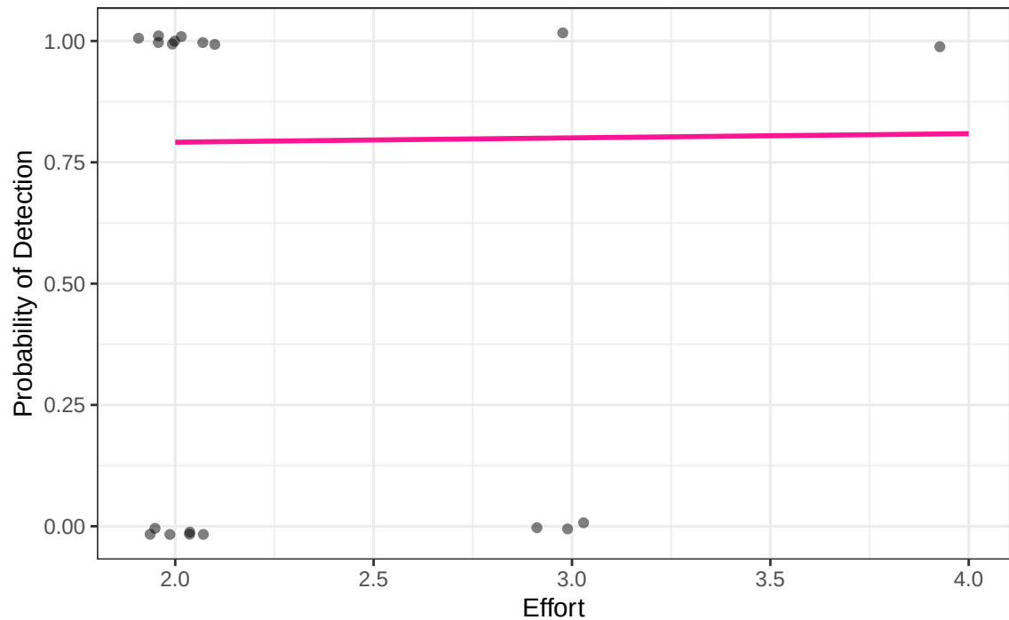
Logistic Regression Curve: Effort
