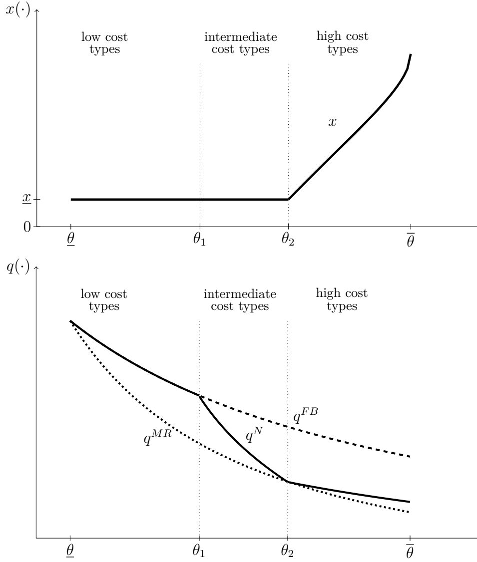
Figure 2: The mechanism of Theorem 1 for the parameter values of Example 1. q^N(\cdot) is the quantity without inspection. q^{MR}(\cdot) is the optimal quantity in a setting where inspection is not feasible (see Mussa and Rosen (1978)).
