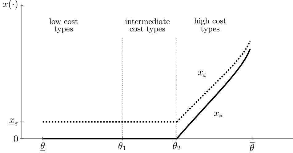
Figure 3: The inspection probability x_*(\cdot) of Theorem 2.
