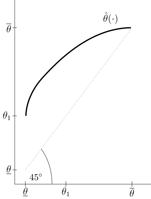
Figure 1: Binding incentive constraints in the constrained optimal mechanism of Example 1. Type \theta on the vertical axis is indifferent between reporting his type truthfully and reporting \hat{\theta}(\theta) . The dotted line shows the binding incentive constraints in the optimal mechanism when inspection is infeasible and, consequently, local incentive constraints bind.
