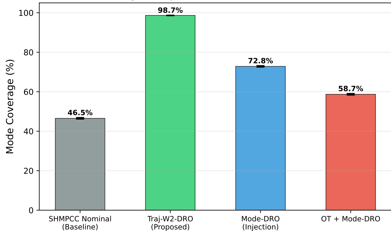
Mode Coverage Comparison (2000 rollouts, 95% Wilson CI)
