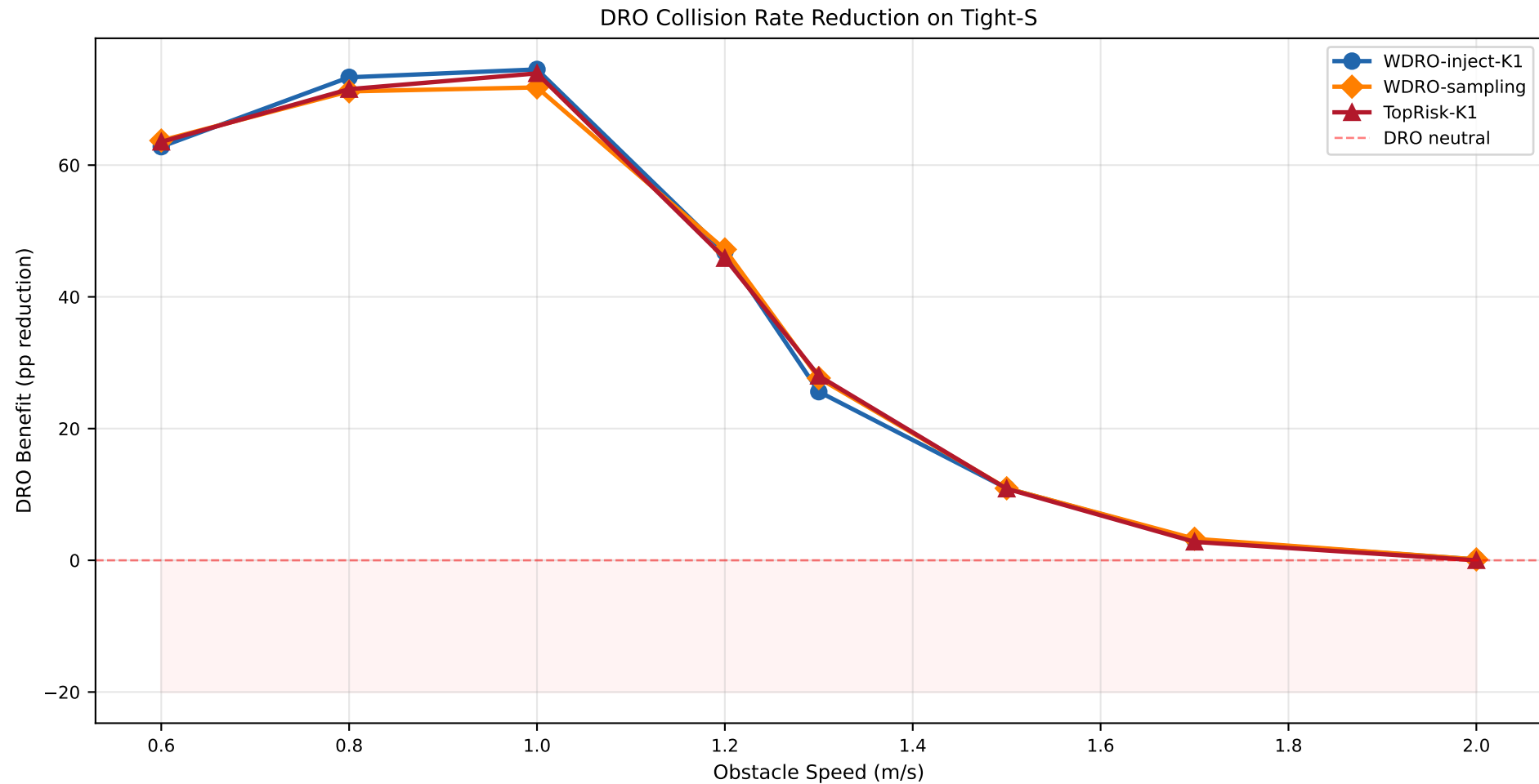
F10: DRO Benefit vs Speed (Tight-S, N=1500)
