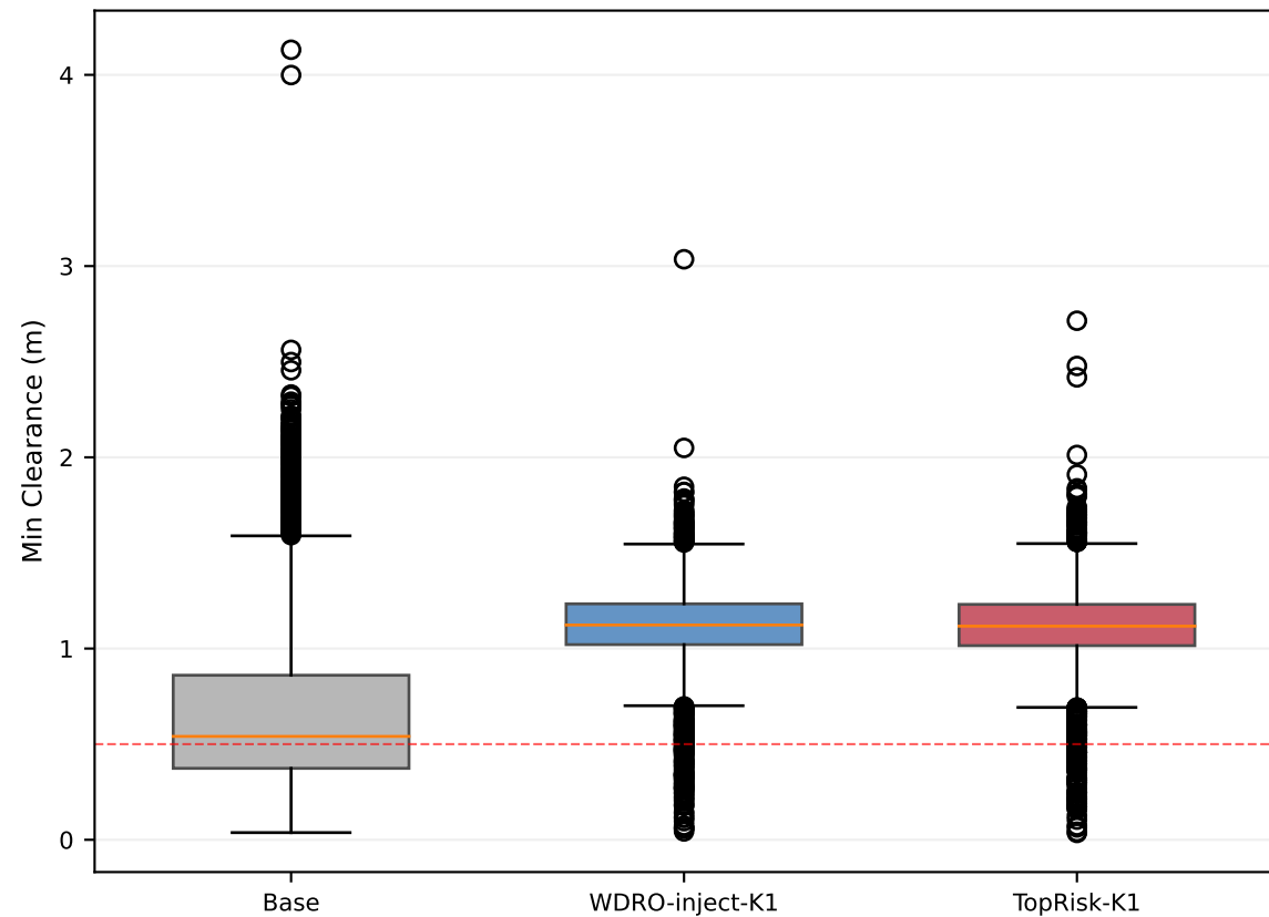
Oncoming: Clearance Distribution
