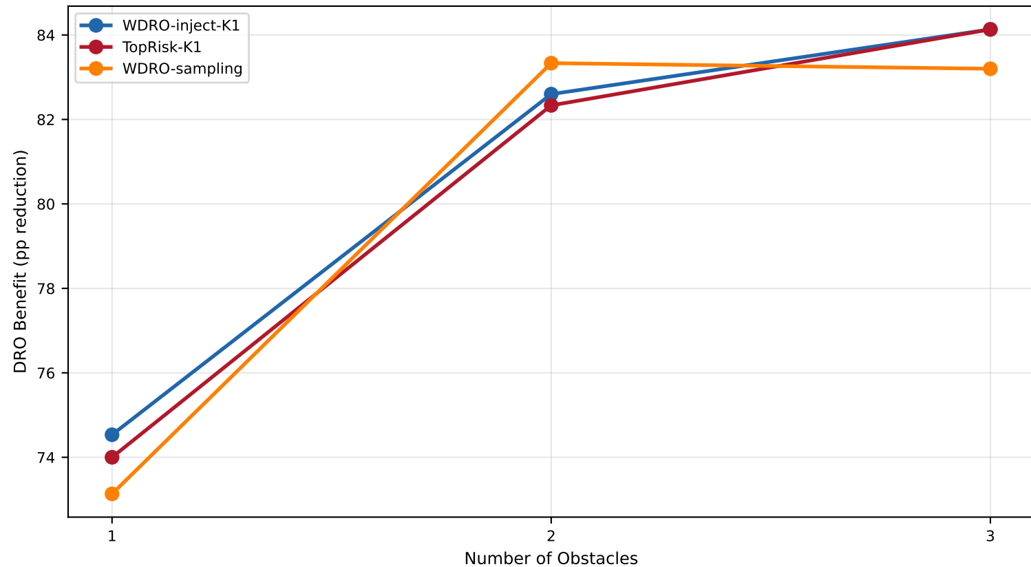
DRO Collision Rate Reduction vs # Obstacles
