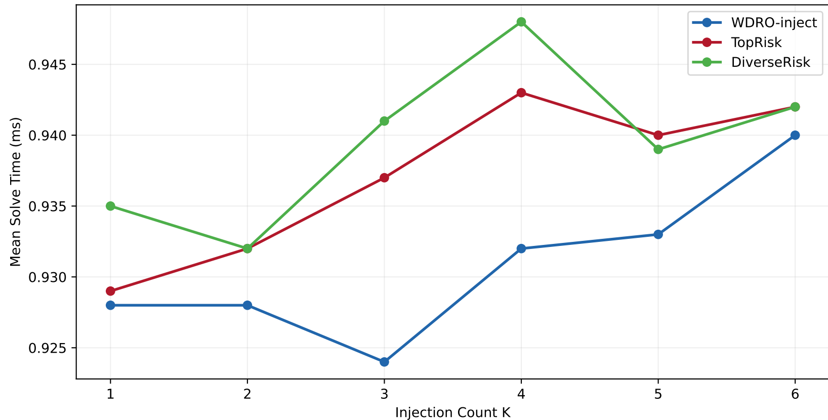
Solve Time vs K (S-curve condition)
