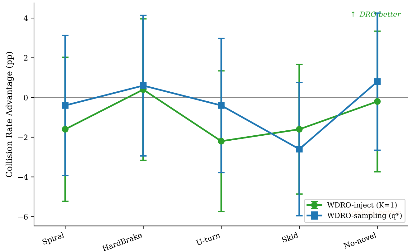
(b) DRO Advantage Over TopRisk-K1
