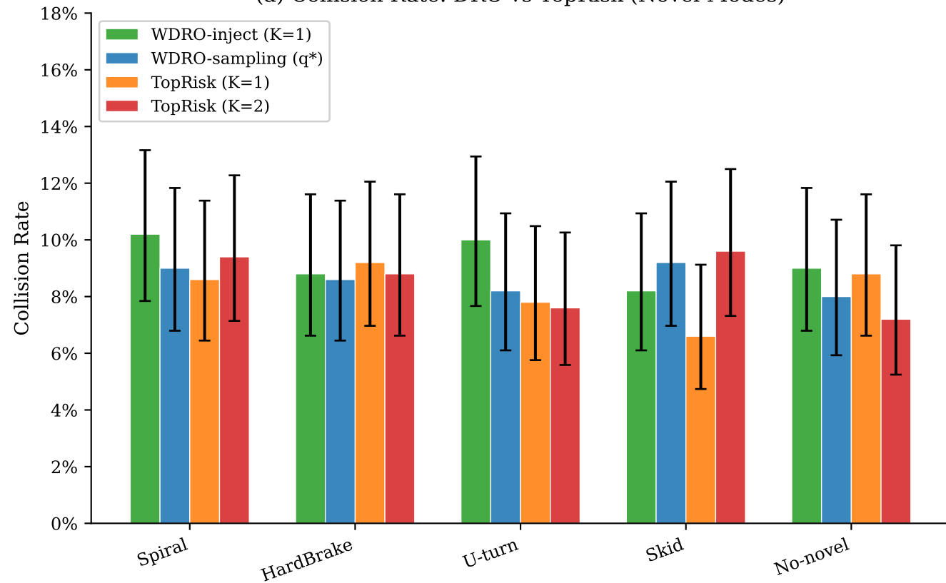
(a) Collision Rate: DRO vs TopRisk (Novel Modes)
