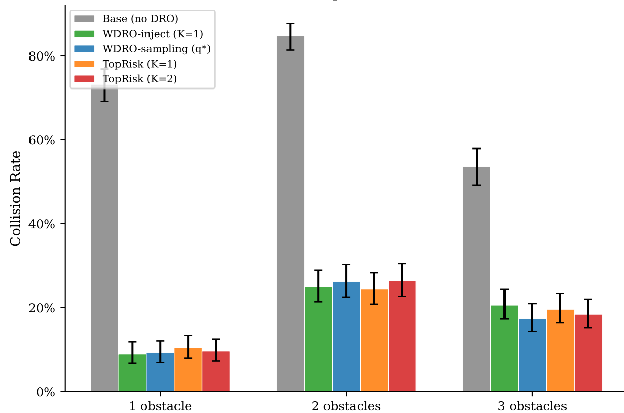
(a) Collision Rate: Sharp Swerve + Multi-Obstacle
