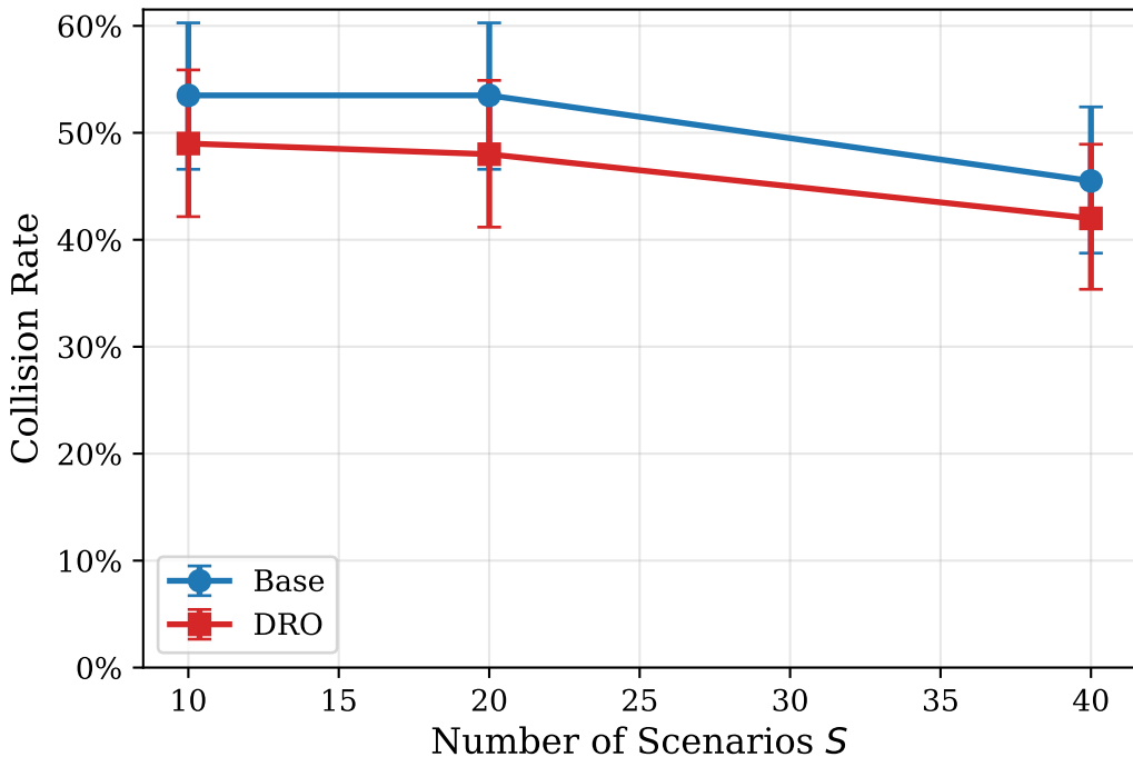
H2: Collision Rate — DRO vs Base (paired MC)
