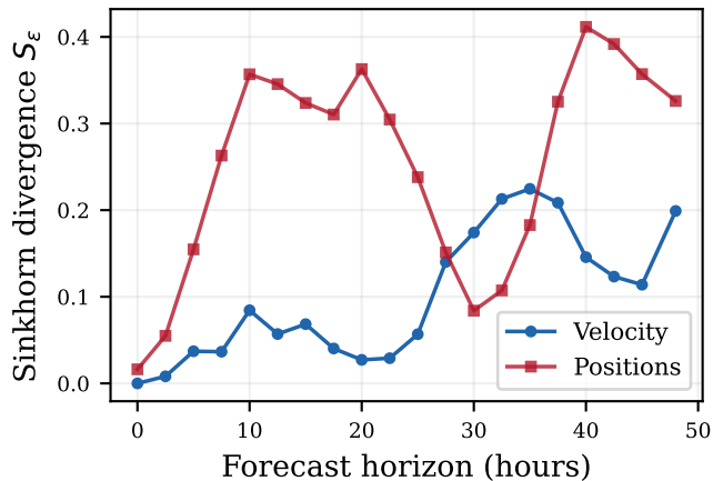
(b) Sinkhorn divergence S_\epsilon
