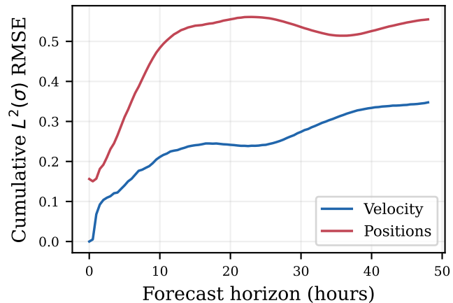
(c) Cumulative RMSE (velocity +37%)
