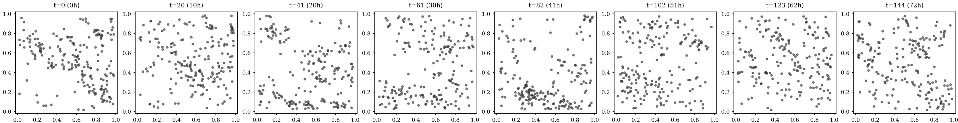
GOES-16 Great Plains 72h — cloud particle evolution (IR band C13)
