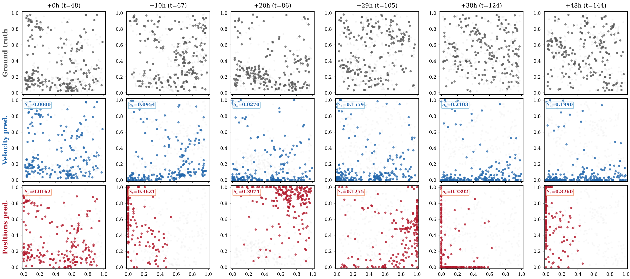
GOES-16 Great Plains 72h — shared HPs ( \rho=0.9 , \alpha=0.9 , \lambda=0.01 ) Velocity map RMSE = 0.2480, Positions map RMSE = 0.6214 (velocity +60.1%)
