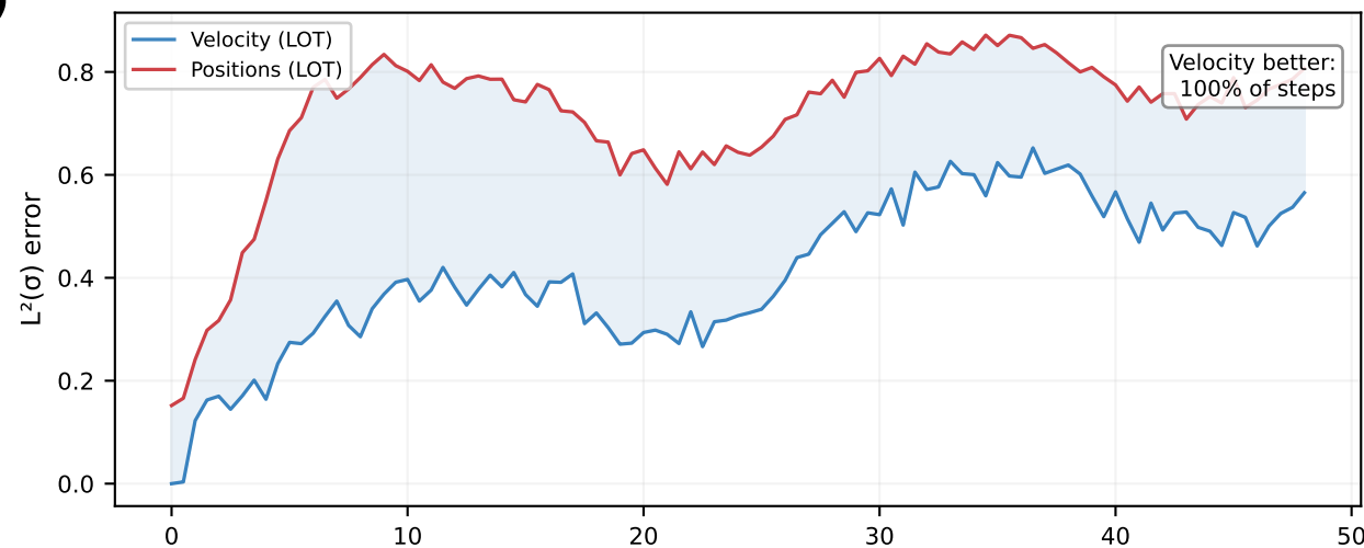
GP Summer, Full 72h — Extended Horizon \rho=0.9 , \alpha=0.9 , \lambda=0.01 , N=200 , R=200
