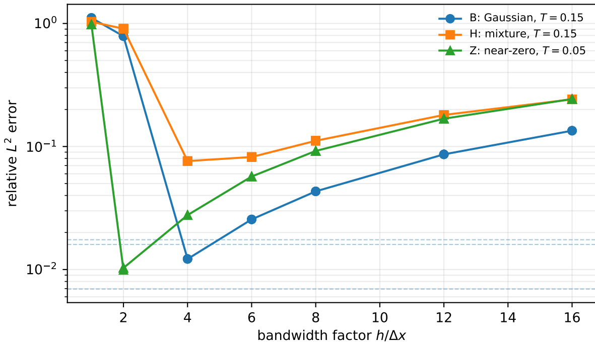
Bandwidth sweep: U-shaped regularization curves (smoothed-log)
