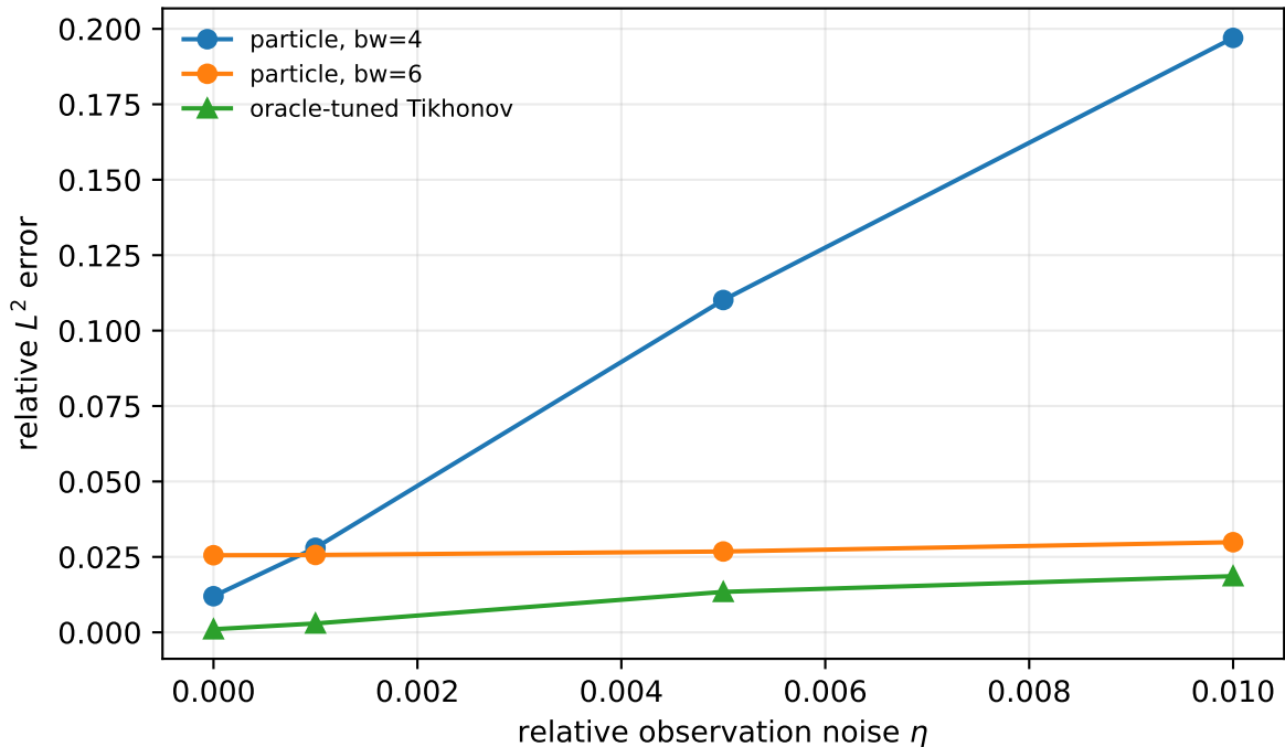
Noise robustness: larger bandwidth trades bias for stability
