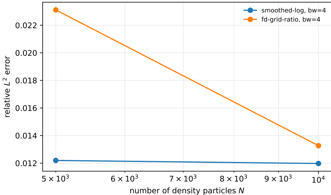
Particle-count refinement on clean Gaussian data (Test B)
