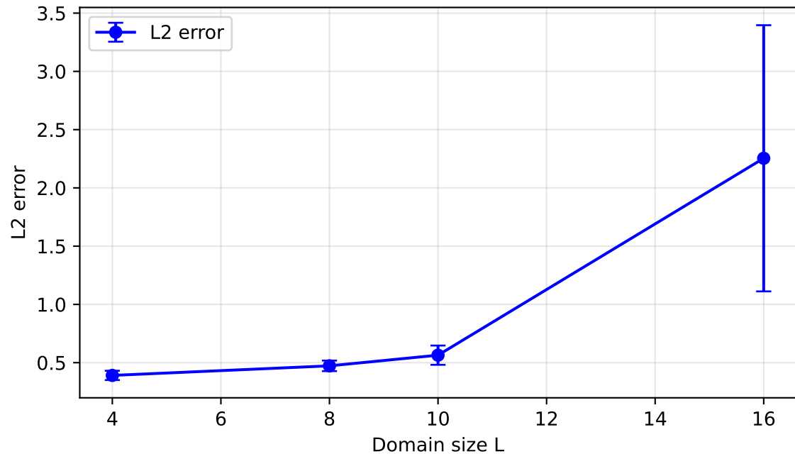
Cole-Hopf: error vs domain size Fixed N=400
