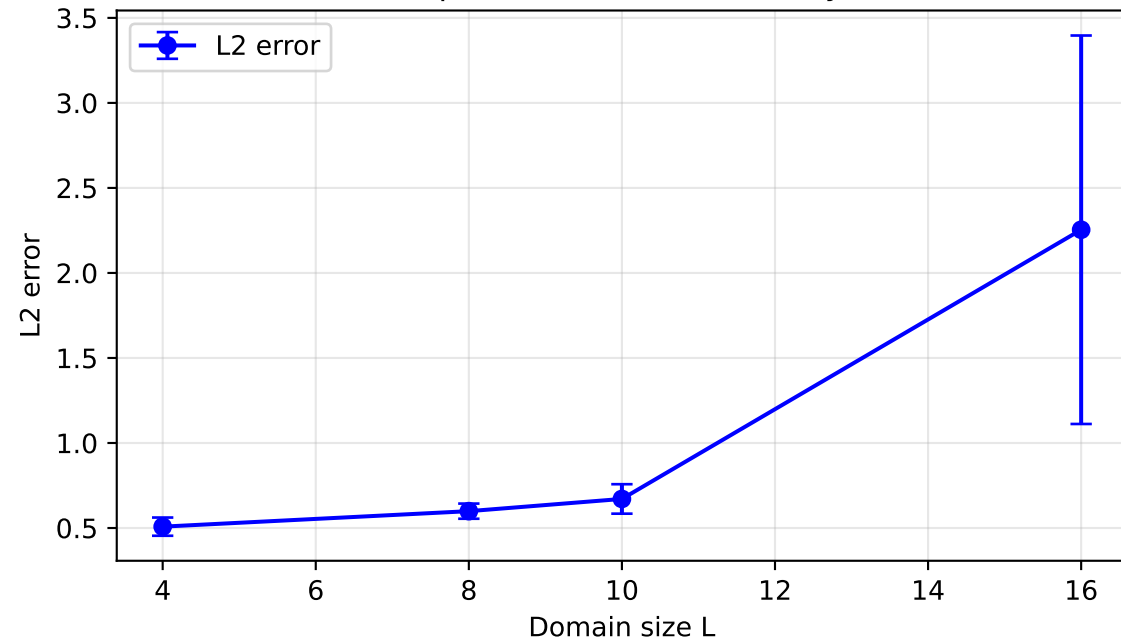
Cole-Hopf: error vs domain size Proportional N (fixed density)
