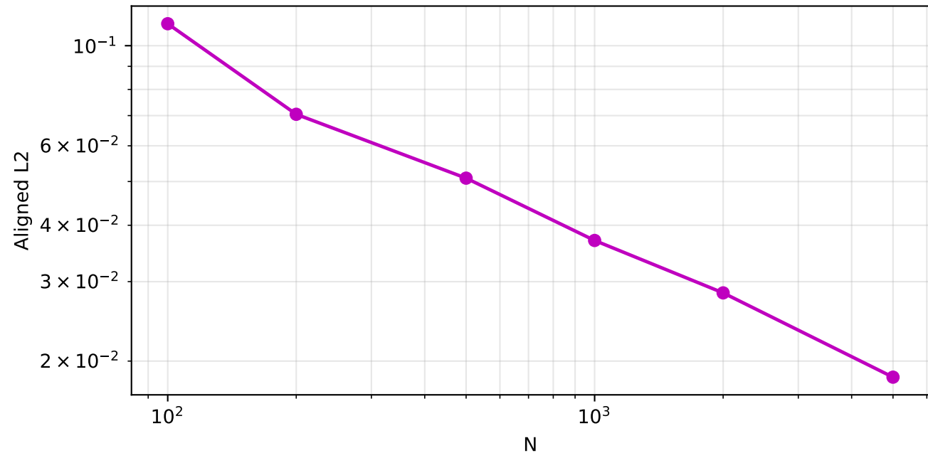
FHN: aligned-profile error vs N slope=-0.444 CI=[-0.475,-0.414]
