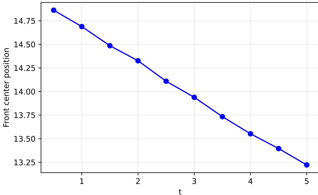
FHN: front center vs time (N=5000)
