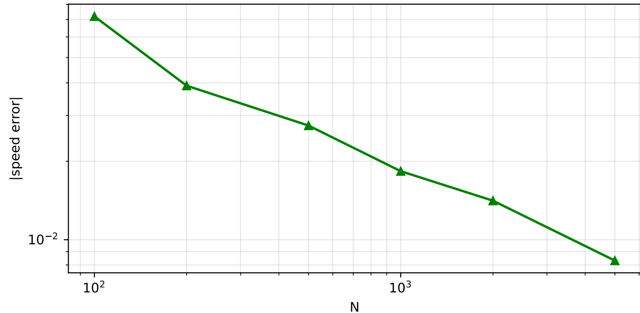
FHN: front speed error vs N slope=-0.524 CI=[-0.607,-0.441]
