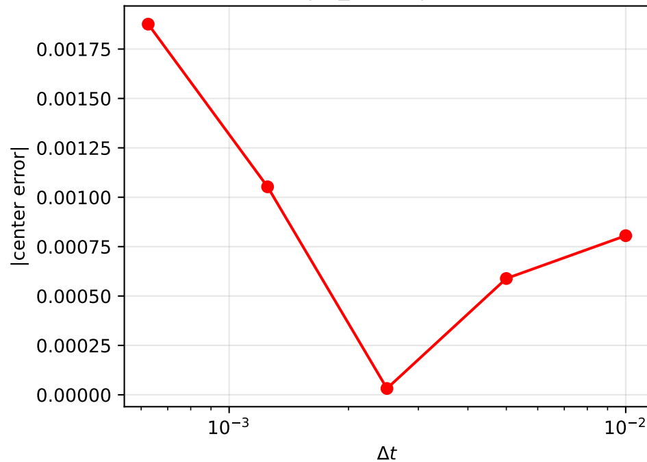
Center error |x_{\text{c\_fit}} - x_{\text{c}}| vs dt (N=6400)
