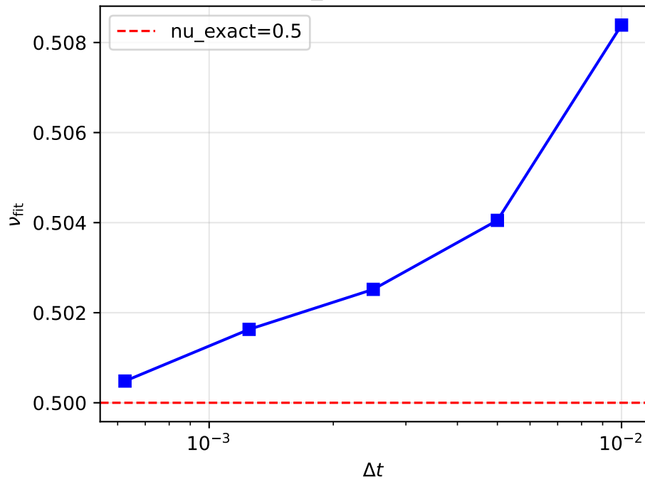
Fitted nu_fit vs dt (N=6400)
