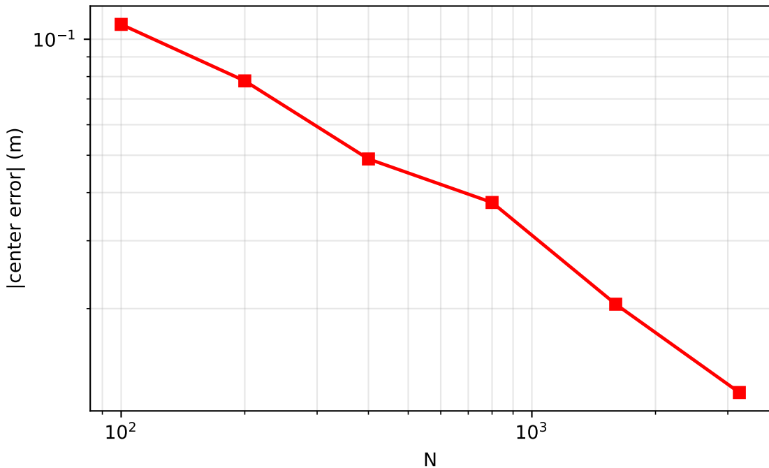
Traveling shock: center error vs N (T=1.0)
