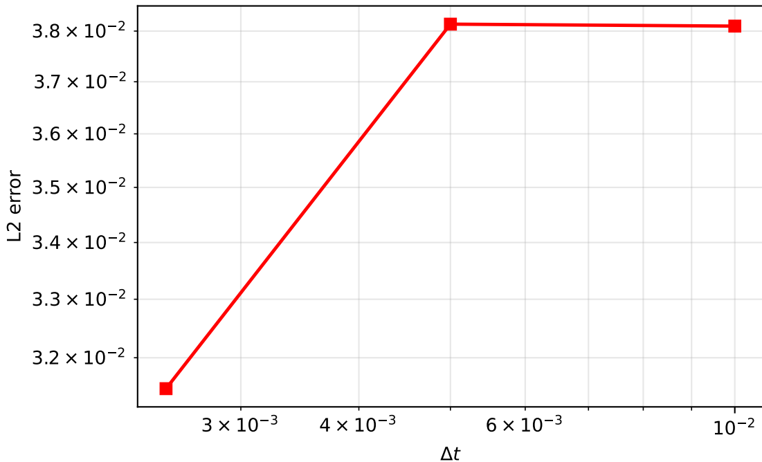
Traveling shock: L2 vs dt (N=1600, T=1.0)
