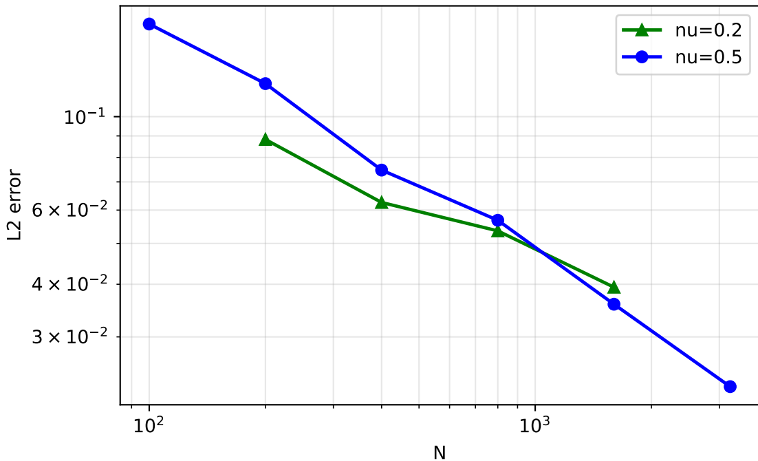
Traveling shock: sharp layer comparison (T=1.0)
