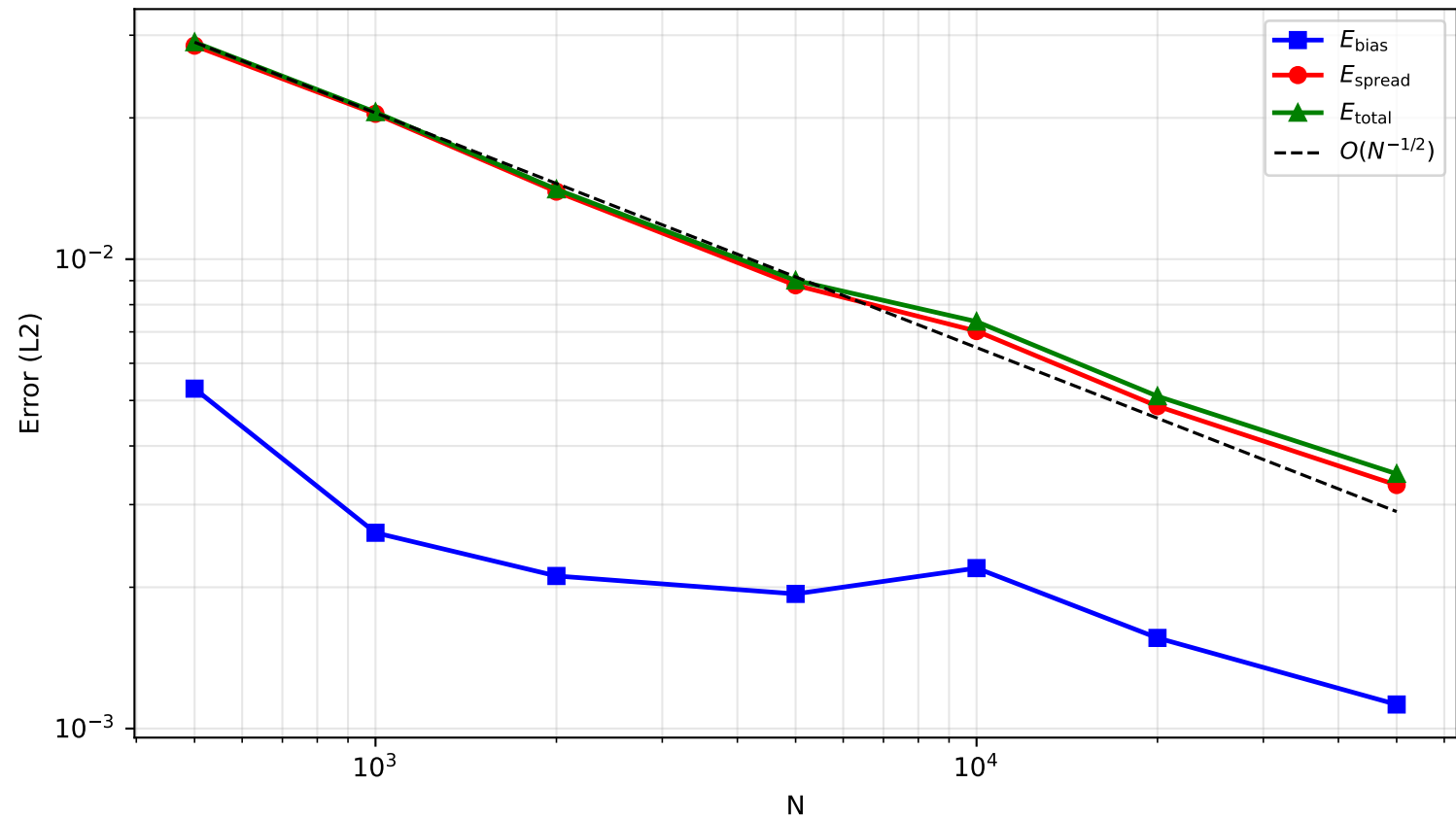
Heat GRW: bias/spread/total vs N total slope=-0.457 95%CI=[-0.483,-0.425]
