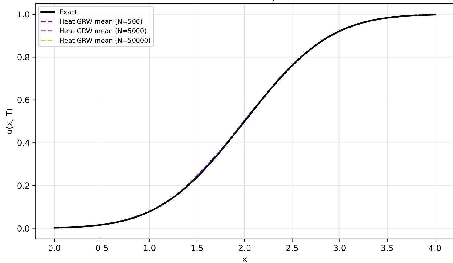
Heat GRW ensemble-mean profiles vs exact
