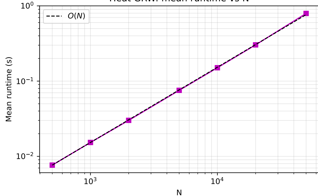
Heat GRW: mean runtime vs N
