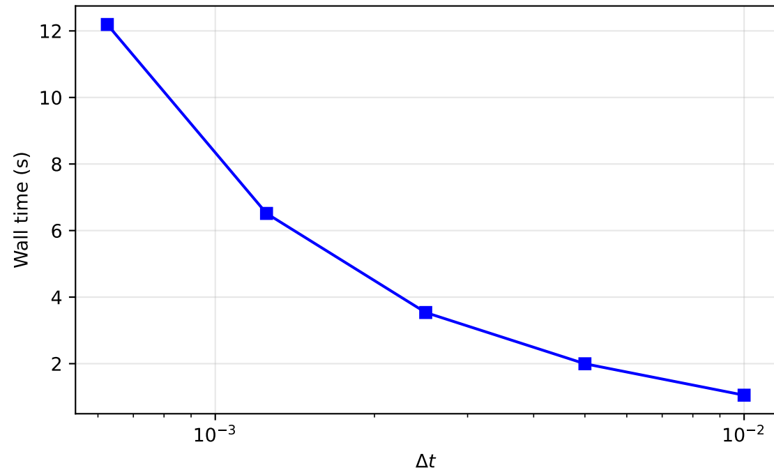
GBMC total runtime (40 seeds) vs dt N=6400
