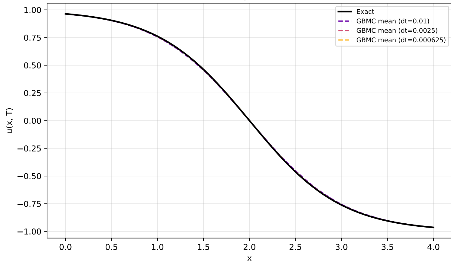
GBMC ensemble-mean profiles vs exact N=6400
