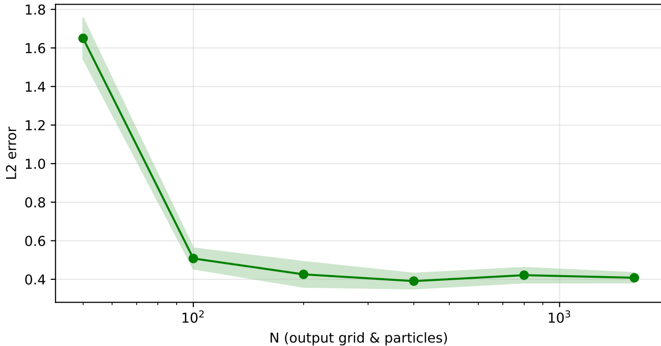
Cole-Hopf: error vs output grid resolution
