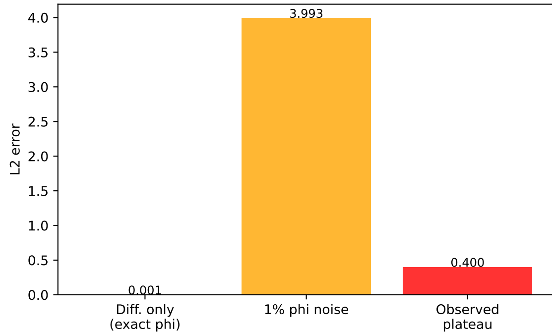
Cole-Hopf plateau: error source decomposition
