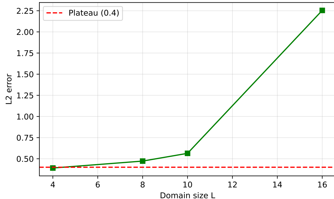
Error vs domain size (fixed N=400)
