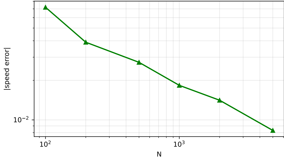
FHN: front speed error vs N slope=-0.524
