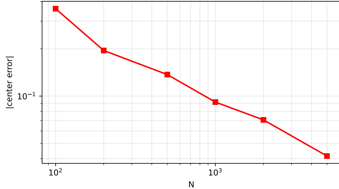
FHN: front center error vs N slope=-0.524
