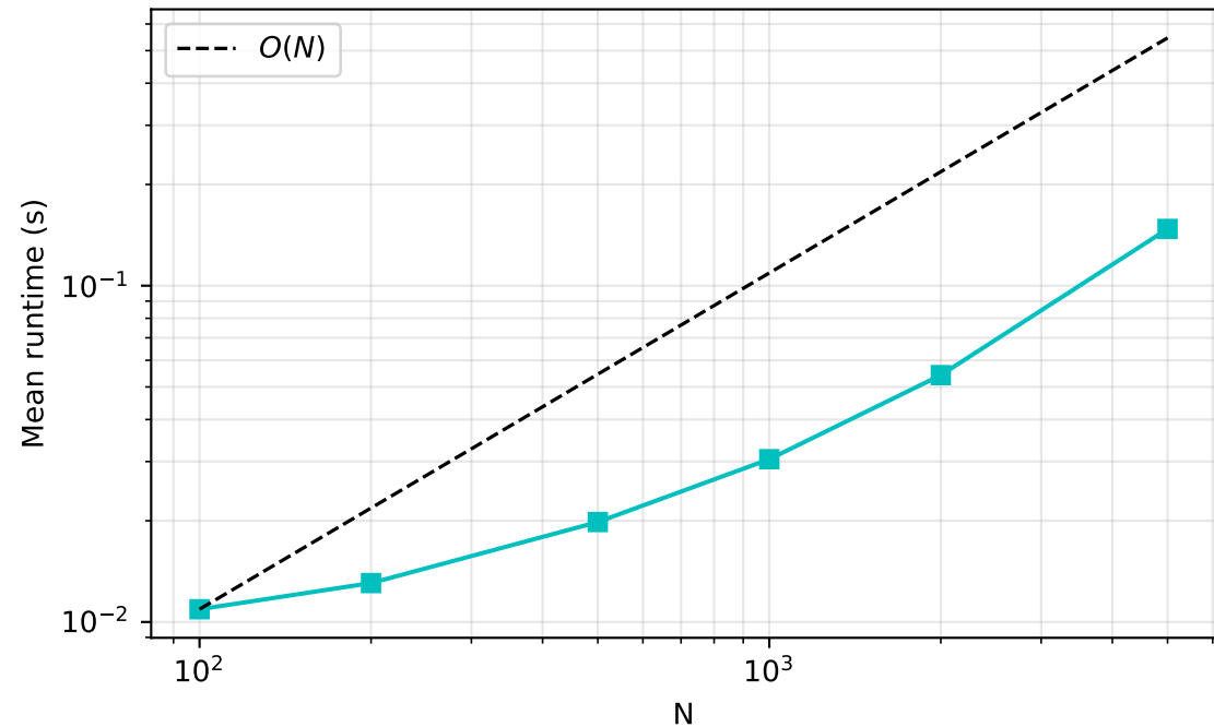
FHN: mean runtime vs N
