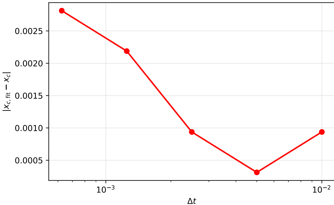
GBMC shock-center error vs dt N=6400
