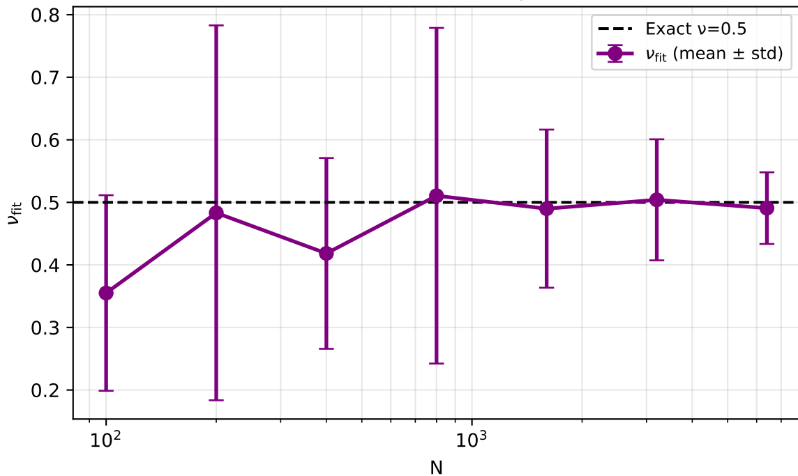
GBMC: fitted viscosity vs N
