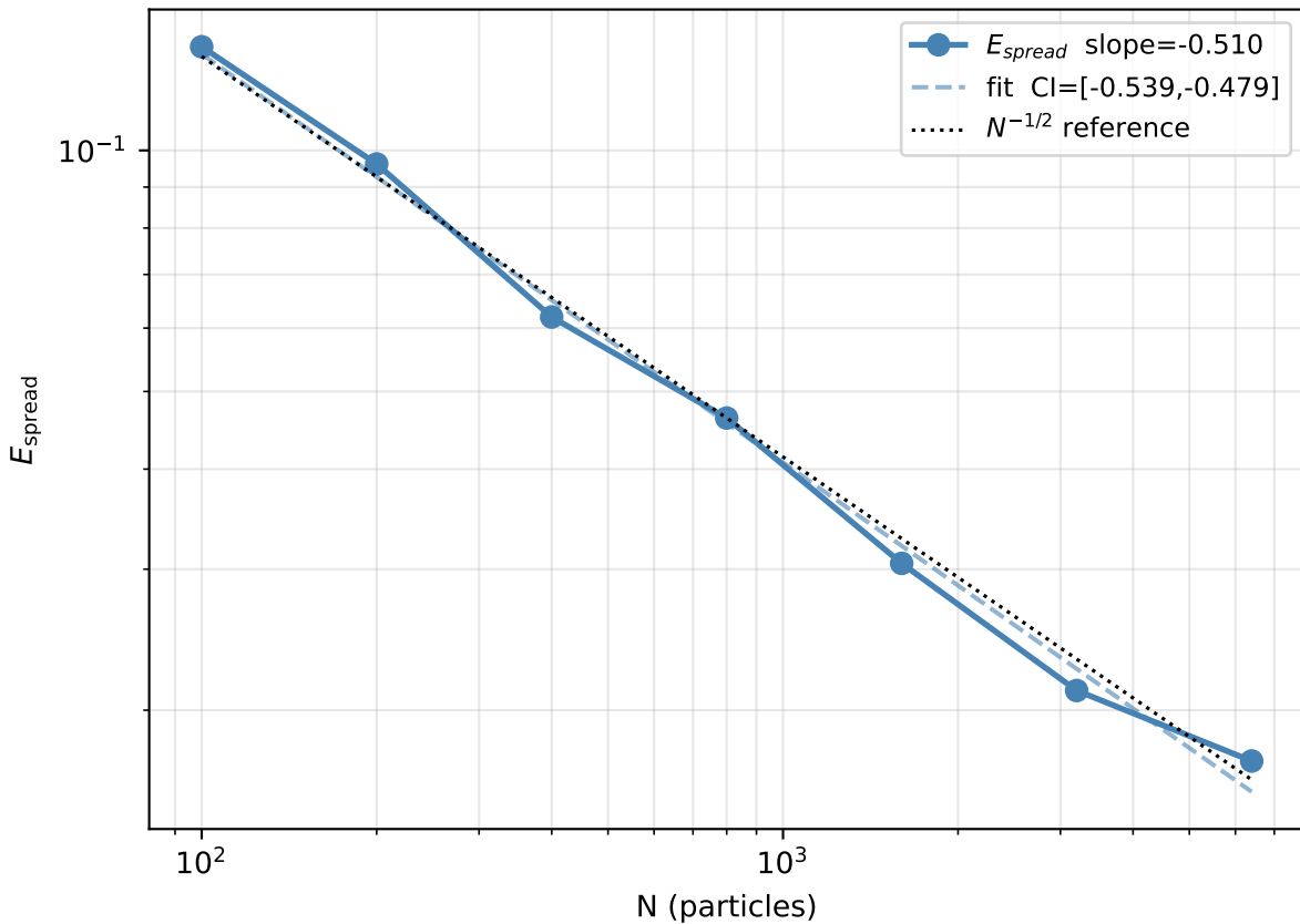
GBMC production: stochastic spread vs N
