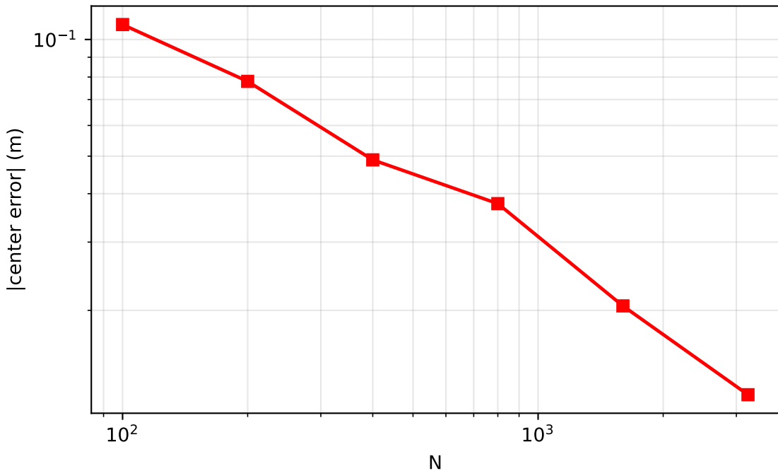
Traveling shock: center error vs N (T=1.0)
