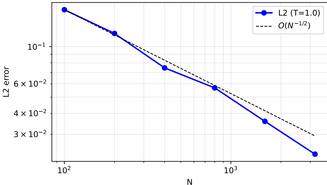
Traveling shock: L2 vs N (nu=0.5, c=0.5, T=1.0) Fitted slope=-0.569 CI=[-0.604,-0.519]
