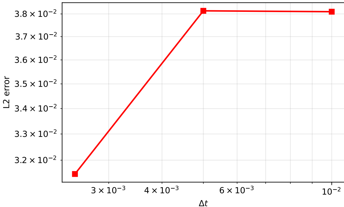
Traveling shock: L2 vs dt (N=1600, T=1.0)
