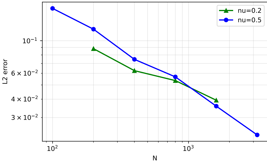
Traveling shock: sharp layer comparison (T=1.0)
