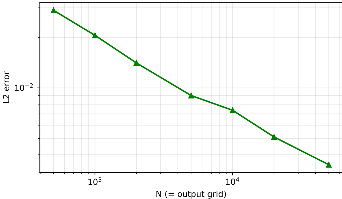
Heat GRW: total error vs N (=output grid size) Note: output grid resolution = N (coupled)
