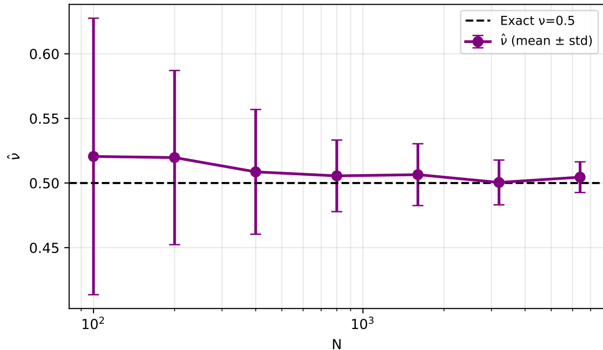
RB--GBMC: fitted viscosity vs N
